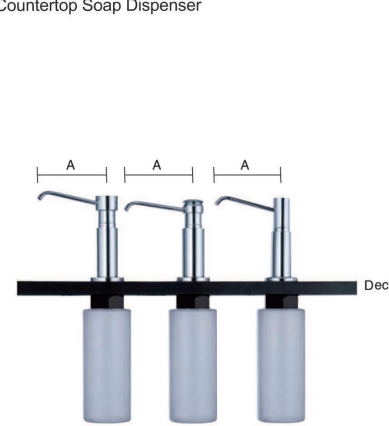
Brass 6880-26-80CP Each dispense:1.0cc Capacity:360ml A:81mm Brass 6803-26-80CP Each dispense:1.0cc Capacity:360ml A:81mm Brass 6759-26-80CP Each dispense:1.0cc Capacity:360ml A:81mm 6880-26-81CP A:163mm 6803-26-81CP A:163mm 6759-26-81CP A:163mm
