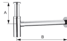
T-Trap 6502-TT-80CP A:170 B:340mm 6502-TT-81CP A:170 B:465mm
