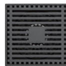
0303-64-79MA Floor Drain Brass Size 100*100 mm Height 51 mm Seal Type Self Seal Brass Flow Rate \geq 15L/Min Outlet OD 40 mm Drain Core 0303-A1-7900
