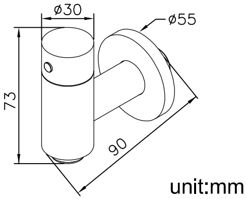
Valve (Water Flow Rate Adjustable)
