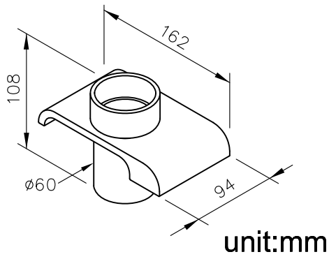
Tumbler Holder
